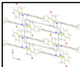
Fig. 2. Part of the crystal structure viewed along the b axis showing hydrogen bonds as dashed lines.
